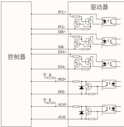
Figure 2 Input signal differential connection method
